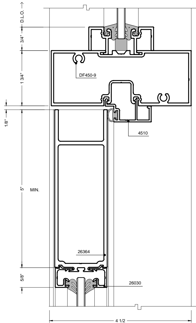
41 WS DOOR HEADER W/ TRANSOM (STANDARD) OFFSET PIVOT & BUTT HINGE FOR CONTINUOUS GEAR HINGE REFER TO 30.1
