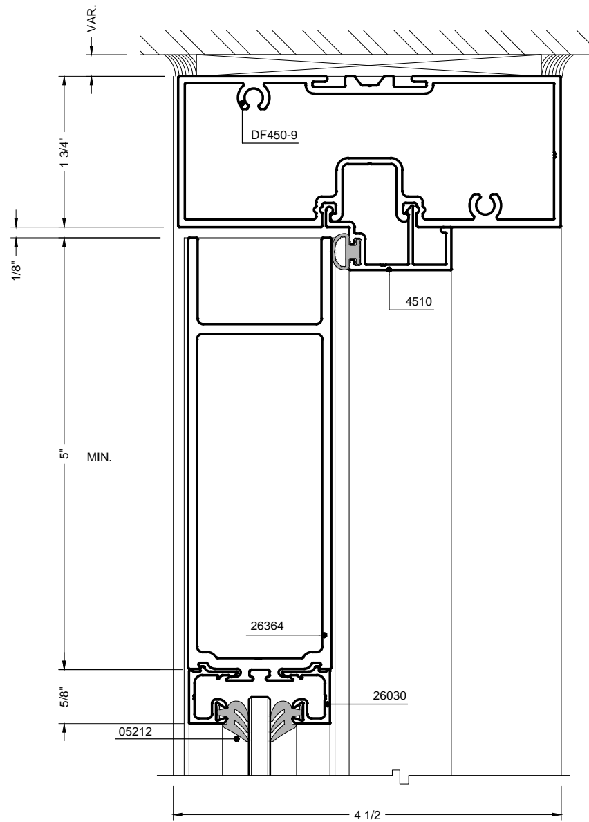
40 WS DOOR HEADER (STANDARD) OFFSET PIVOT & BUTT HINGE FOR CONTINUOUS GEAR HINGE REFER TO 30.1
