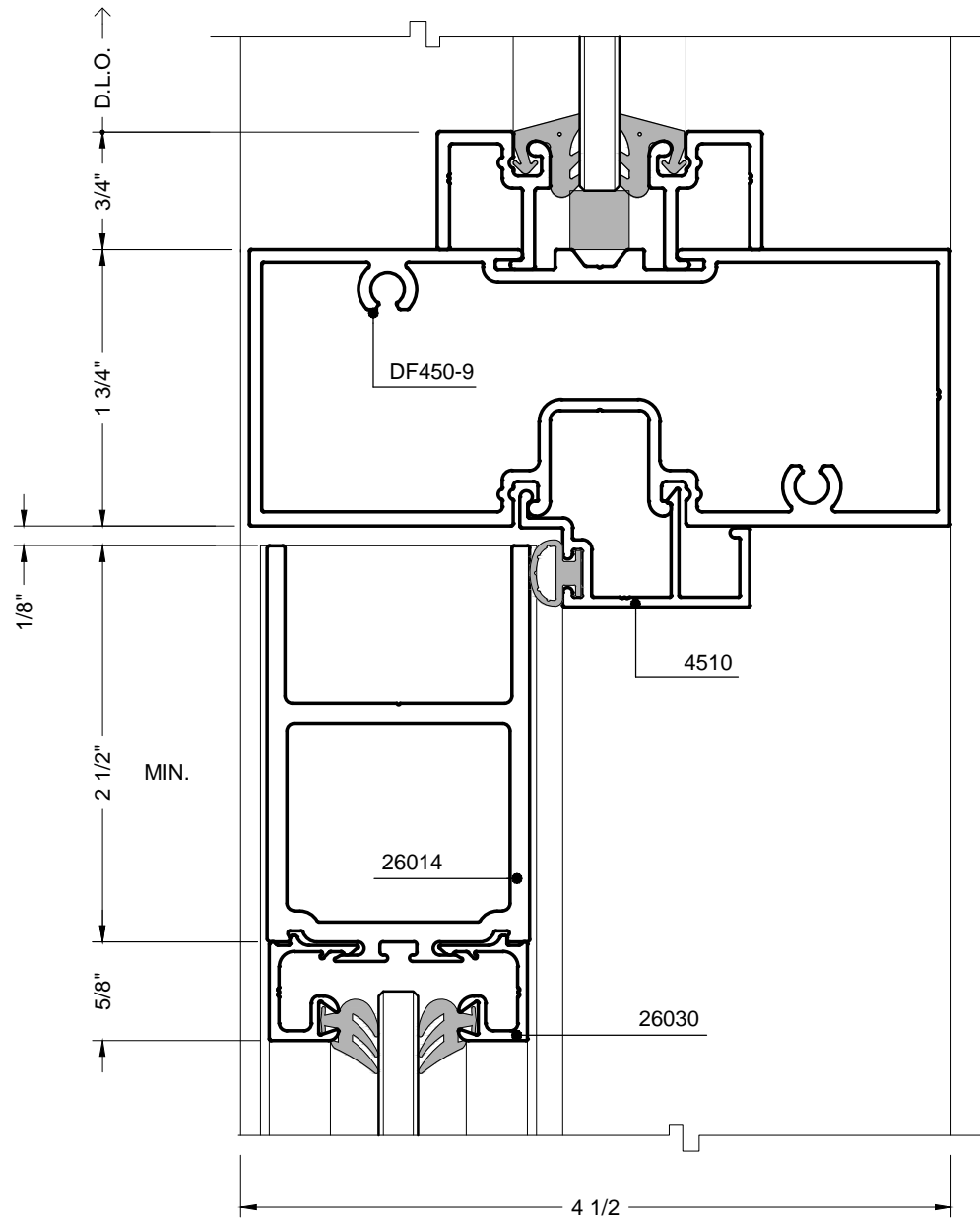
41 DOOR HEADER W/ TRANSOM (STANDARD) OFFSET PIVOT & BUTT HINGE FOR CONTINUOUS GEAR HINGE REFER TO 30.1
