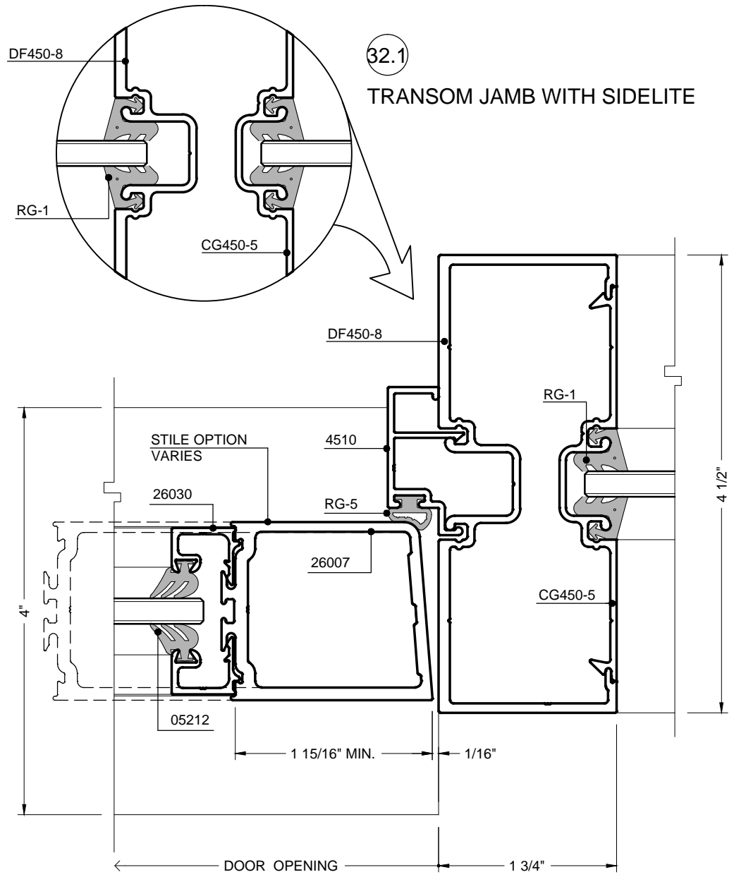
32 DOOR JAMB (STANDARD) OFFSET PIVOT & BUTT HINGE FOR CONTINUOUS GEAR HINGE REFER TO 30.1
