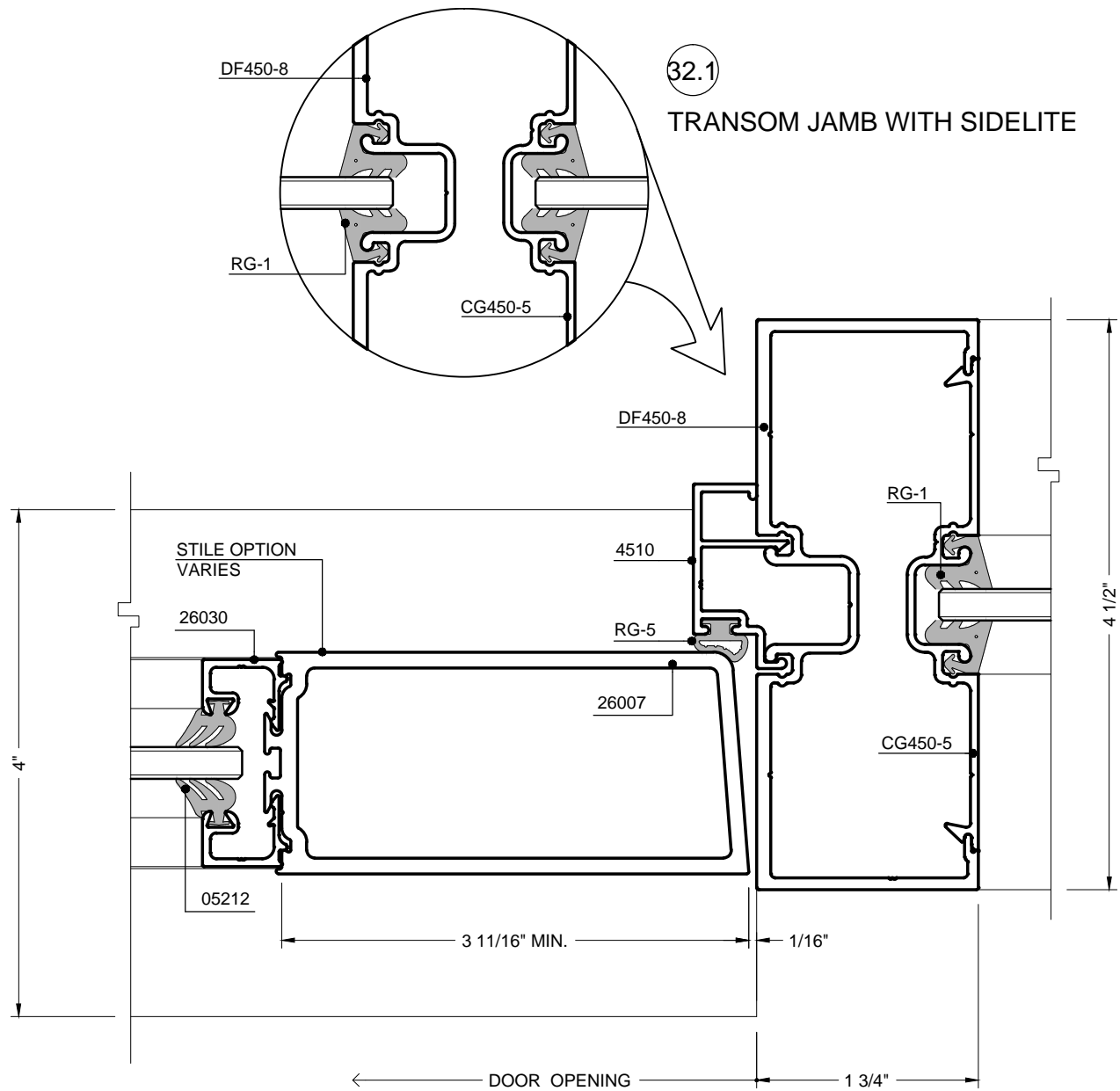
32 MS DOOR JAMB (STANDARD) OFFSET PIVOT & BUTT HINGE FOR CONTINUOUS GEAR HINGE REFER TO 30.1
