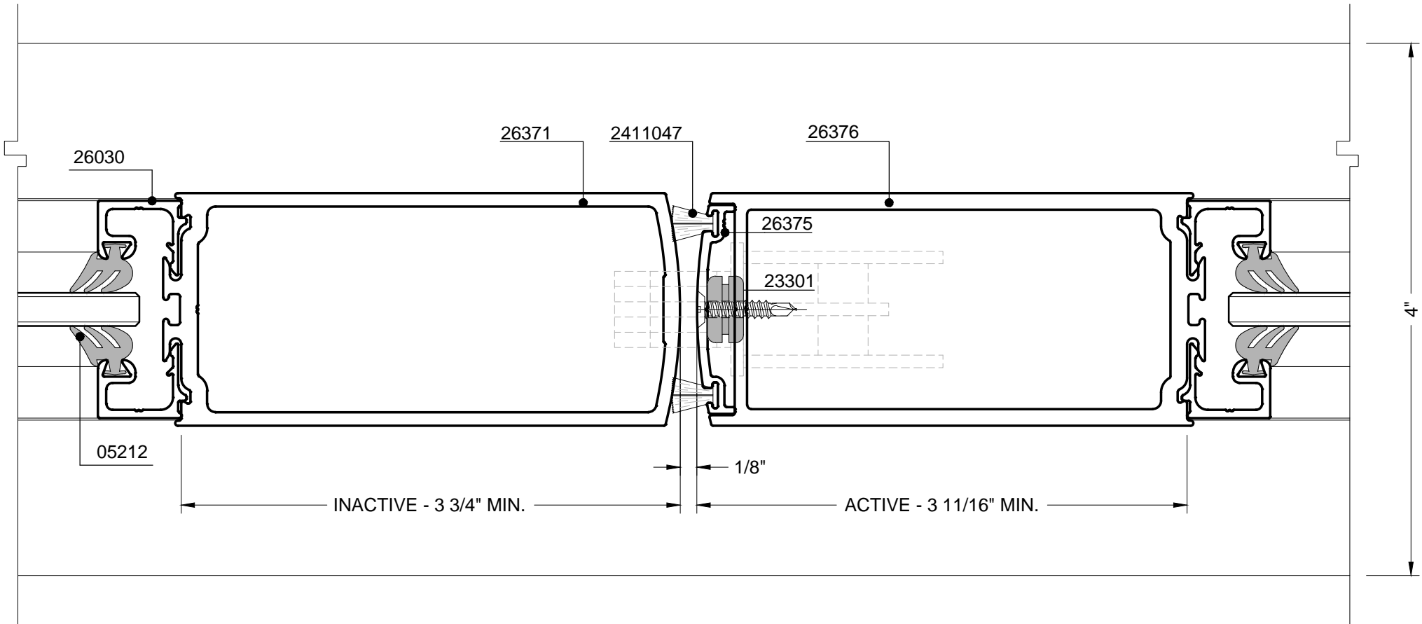
31 MS MEETING STILES (STANDARD) SERIES-200: AS SHOWN
